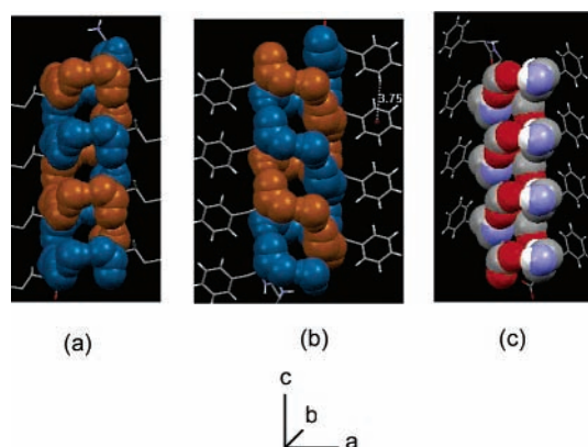
Figure 3. (a) and (b) Space-filling model of the supramolecular double helical architecture of peptides 2 and 3 . CH- \pi interaction is also shown. (c) Supramolecular single helix formation of peptide 4 along the crystallographic c -axis.
